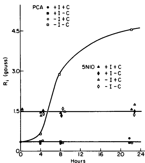
FIGURE 3 Empirical motion parameter ( R_1 ) plotted vs. time under different growth conditions. The structures and properties of the spin labels PCA and 5N10 are described in the text. Abbreviations: C, cycloheximide; I, inositol.
